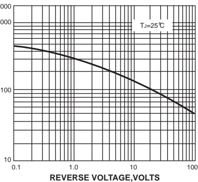
FIG. 5-TYPICAL JUNCTION CAPACITANCE
