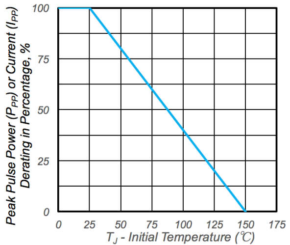
Fig.2 - Pulse Derating Cure
