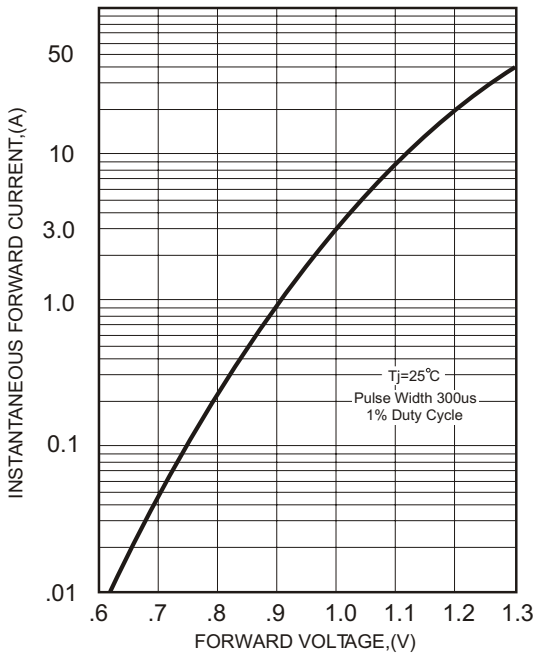
FIG.1-TYPICAL FORWARD CHARACTERISTICS
